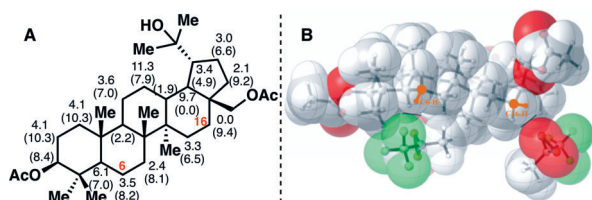
Figure 3. Analysis of site selectivities on 12 for TFDO. a) Relative activation enthalpies for equatorial C–H abstraction by DMDO ( \Delta\Delta H^\ddagger ) and relative stabilities of the free radicals ( \Delta\Delta E , in parentheses) ( \text{kcal mol}^{-1} ). b) Juxtaposition of space-filling models of TFDO approaching C6–H and C16–H in 12 , to indicate the steric effects disfavoring C–H abstraction from C6–H. The relative orientations of TFDO and 12 were determined from the transition-state geometries shown in Figure S13 in the Supporting Information.
