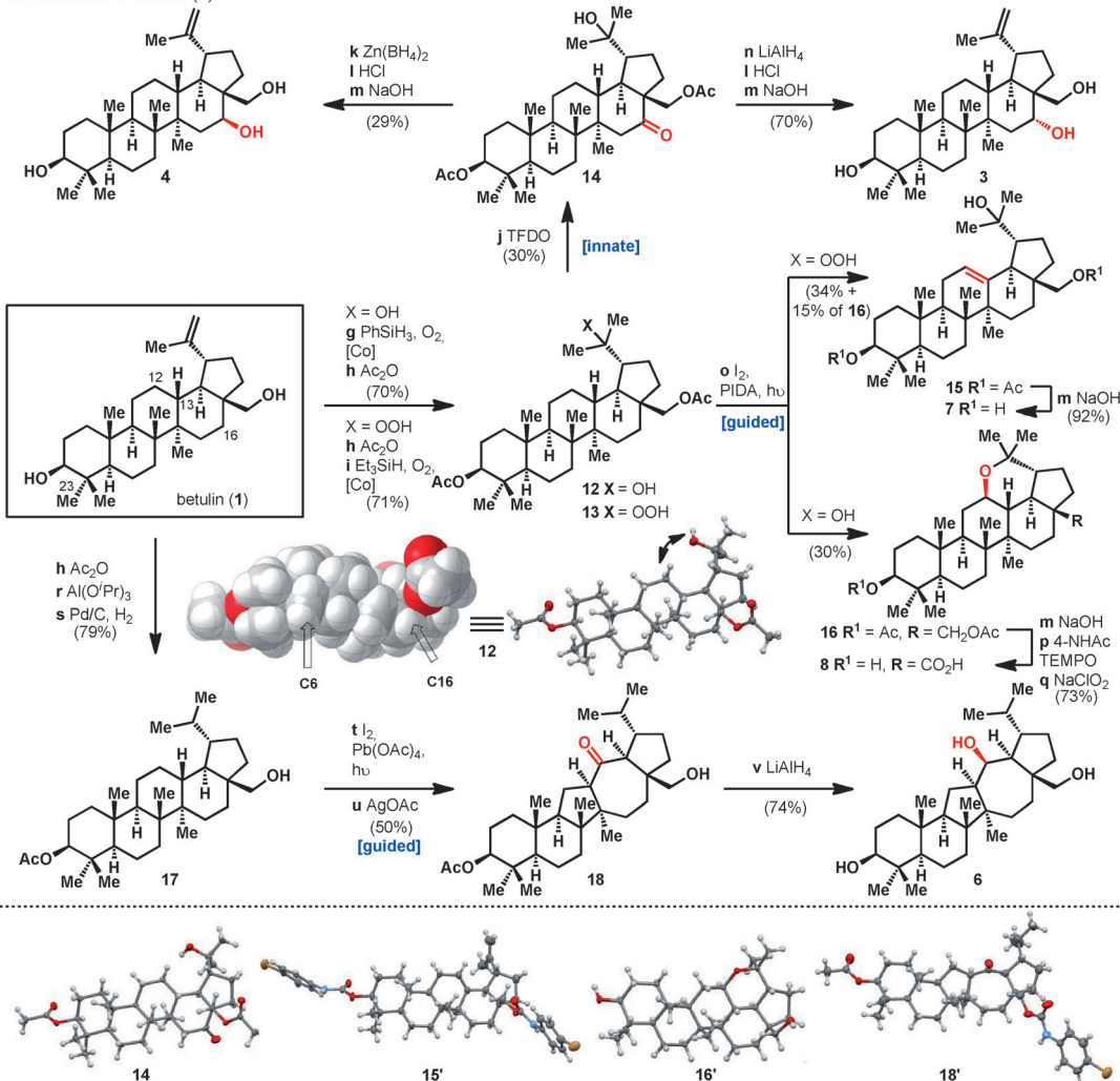
Figure 2. Divergent synthesis of oxidized compounds from a) betulinic acid and b) betulin. Reagents and conditions: a) \text{BnBr} , \text{K}_2\text{CO}_3 , 60^\circ\text{C} , 3.5 h, 92%; b) 1 mol% [\{\text{Ir}(\text{cod})\text{OMe}\}_2] , \text{Et}_2\text{SiH}_2 , RT, 12 h; c) 2 mol% [\{\text{Ir}(\text{cod})\text{OMe}\}_2] , 5 mol% \text{Me}_4\text{Phen} , norbornene, 120^\circ\text{C} , 36 h; d) \text{H}_2\text{O}_2 , \text{KHCO}_3 , 50^\circ\text{C} , 12 h, 24% (over 3 steps); e) 50 mol% \text{Pd}(\text{OAc})_2 , \text{Et}_3\text{N} , t\text{BuMe}_2\text{SiH} , 60^\circ\text{C} , 2.5 h; f) TBAF, RT, 1.5 h, 70% (over 2 steps); g) Sodium-bis-[N-salicylidene-2-amino-isobutyrate]-cobaltate(III) ( 20 ), \text{PhSiH}_3 , \text{O}_2 , RT, 10 h; h) \text{Ac}_2\text{O} , pyr, RT, 99% (70% for 12 over 2 steps); i) 20 , \text{Et}_2\text{SiH} , \text{O}_2 , RT, 14 h, 71%; j) TFDO, 0^\circ\text{C} , 2 h, 30%; k) \text{Zn}(\text{BH}_4)_2 , RT, 1 h, 80% (1:1 d.r.); l) \text{HCl} , 0^\circ\text{C} ( -41^\circ\text{C} for 4 ); m) \text{NaOH} , RT, 12 h, 72% for 4 (over 2 steps) (70% for 3 (over 3 steps), 92% for 7 ); n) \text{LiAlH}_4 , -95^\circ\text{C} , 1 h; o) \text{I}_2 , PIDA, h\nu , RT, 15 min, 30% of 16 from 14 ; 34% of 15 and 15% of 16 from 13 ; p) 40 mol% 4-NHAcTEMPO, PIDA, RT 3 h; q) \text{NaClO}_2 , \text{NaH}_2\text{PO}_4 \cdot \text{H}_2\text{O} , 2-methyl-2-butene, RT, 2.5 h, 73% (over 3 steps); r) \text{Al}(\text{O}i\text{Pr})_3 , i\text{PrOH} , 100^\circ\text{C} , 1.5 h; s) \text{Pd/C} , \text{H}_2 , RT, 12 h, 79% (over 3 steps); t) \text{I}_2 , \text{Pb}(\text{OAc})_4 , h\nu , RT, 15 min; u) \text{AgOAc} , RT, 20 h, 50% (over 2 steps); v) \text{LiAlH}_4 , 0^\circ\text{C} , 1 h, 74%. cod = 1,5-cyclooctadiene, TBAF = tetra-n-butylammonium fluoride, PIDA = phenyliodine(III) diacetate, TEMPO = 2,2,6,6-tetramethylpiperidin-1-oxyl.
